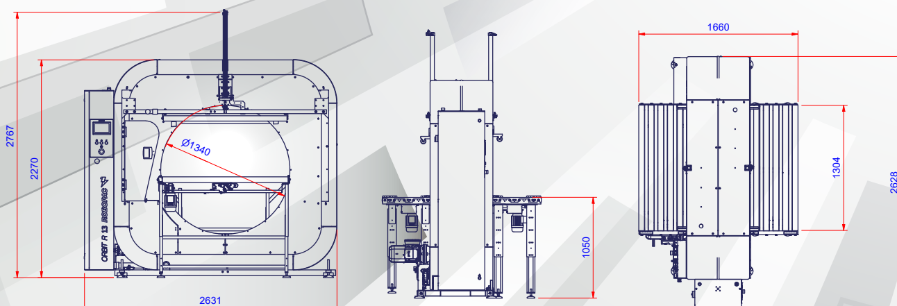
LAYOUT WRAPPY N 13 [mm]
